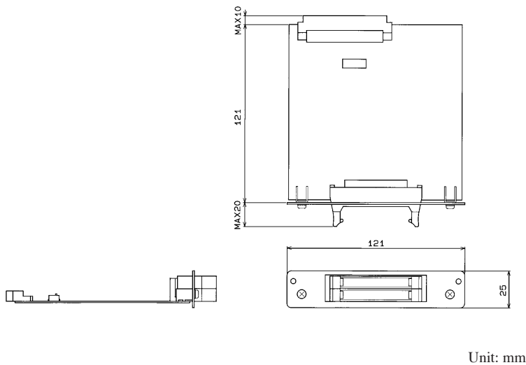
Fig.5-1 PD03M/S-PCR-LA Outer Dimensions
