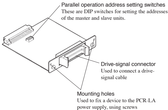
Fig.1-1 PD03M-PCR-LA/PD03S-PCR-LA
