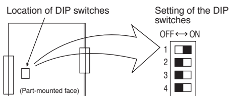
Fig.2-3 DIP Switches on the PCB
