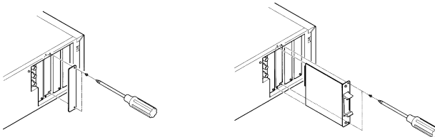
Fig.2-4 Installing a Card
