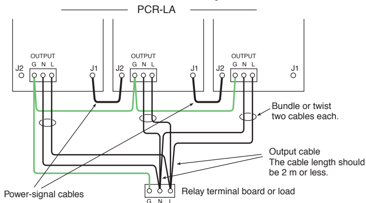
Fig.2-6 Example of the Parallel Connection of PCR-LA Power Supplies
